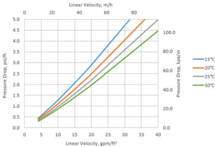
Figure 2 – Pressure drop
