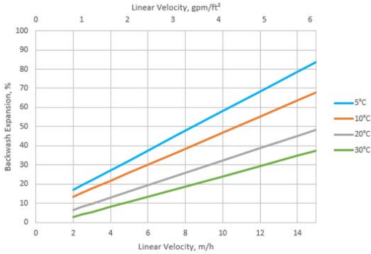
Figure 1 – Backwash expansion
