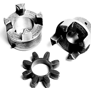
Fig. 6. Shaft coupling
